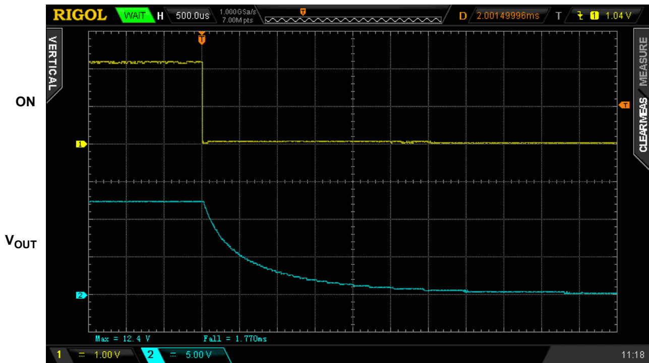
Figure 6. Typical Turn OFF operation waveform for V_{IN} = 12\text{ V} , C_{SLEW} = 10\text{ nF} , C_{LOAD} = 10\text{ }\mu\text{F} , R_{LOAD} = 100\text{ }\Omega
