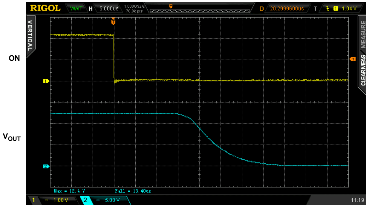
Figure 5. Typical Turn OFF operation waveform for V_{IN} = 12\text{ V} , C_{SLEW} = 10\text{ nF} , no C_{LOAD} , R_{LOAD} = 100\text{ }\Omega
