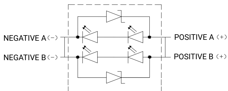
6-V Configuration
