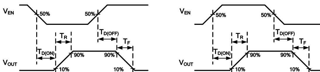
Figure 1. Voltage Waveforms: AP2552/52A (left), AP2553/53A (right)
