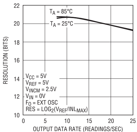
Figure 24. Resolution ( INL_{RMS} \leq 1LSB ) vs Output Data Rate and Temperature
