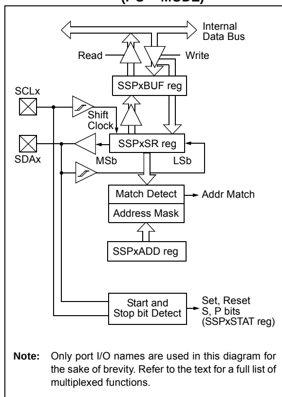
FIGURE 19-7: MSSPx BLOCK DIAGRAM (I 2 C™ MODE)
