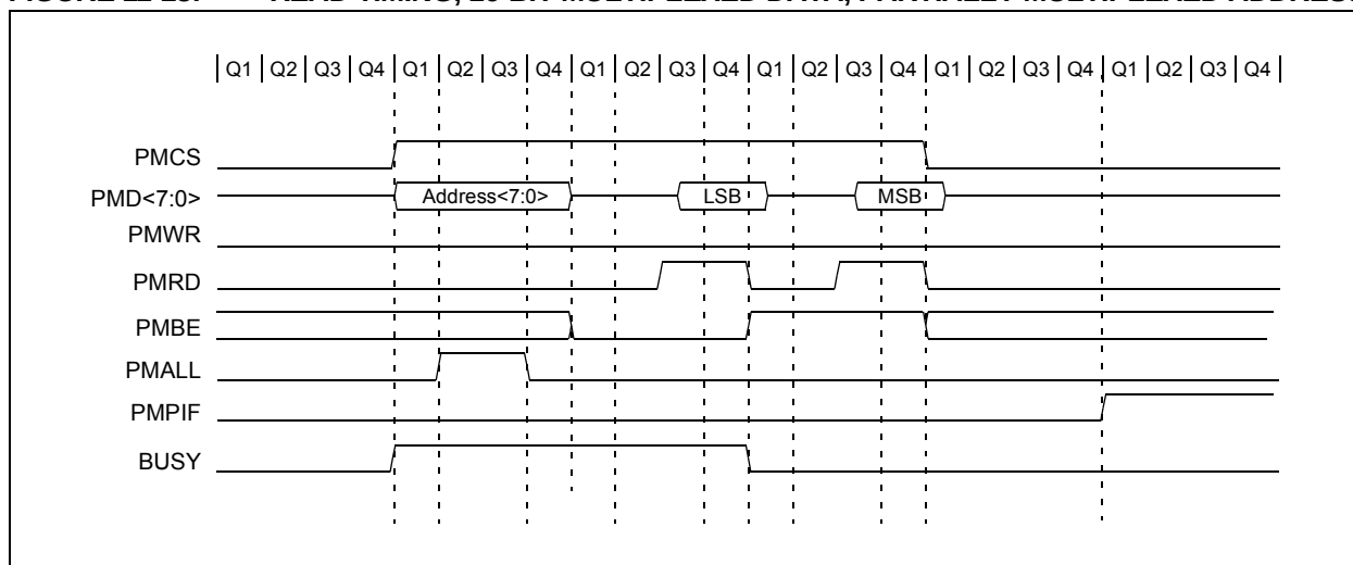
FIGURE 11-23: READ TIMING, 16-BIT MULTIPLEXED DATA, PARTIALLY MULTIPLEXED ADDRESS
