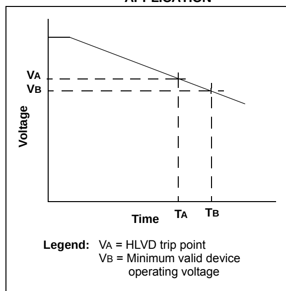
FIGURE 25-4: TYPICAL HIGH/ LOW-VOLTAGE DETECT APPLICATION
