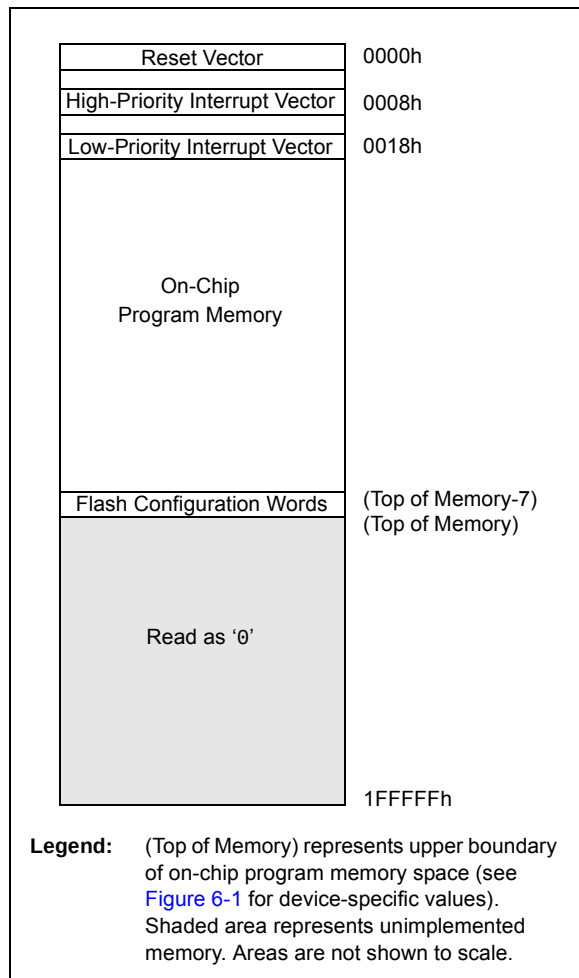
FIGURE 6-2: HARD VECTOR AND CONFIGURATION WORD LOCATIONS FOR PIC18F46J50 FAMILY DEVICES
