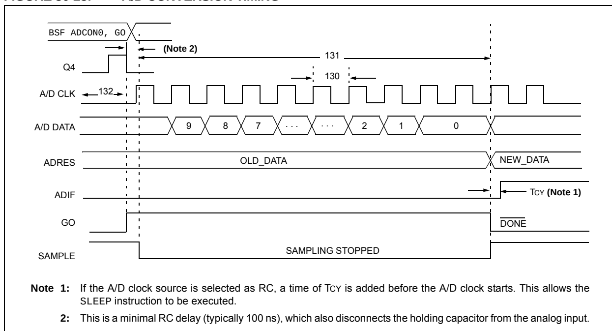
FIGURE 30-23: A/D CONVERSION TIMING
