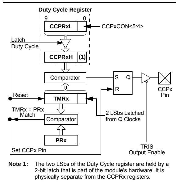
FIGURE 18-3: SIMPLIFIED PWM BLOCK DIAGRAM
