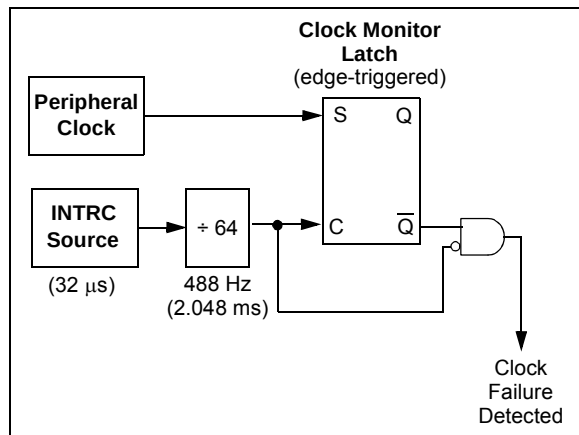
FIGURE 27-4: FSCM BLOCK DIAGRAM
