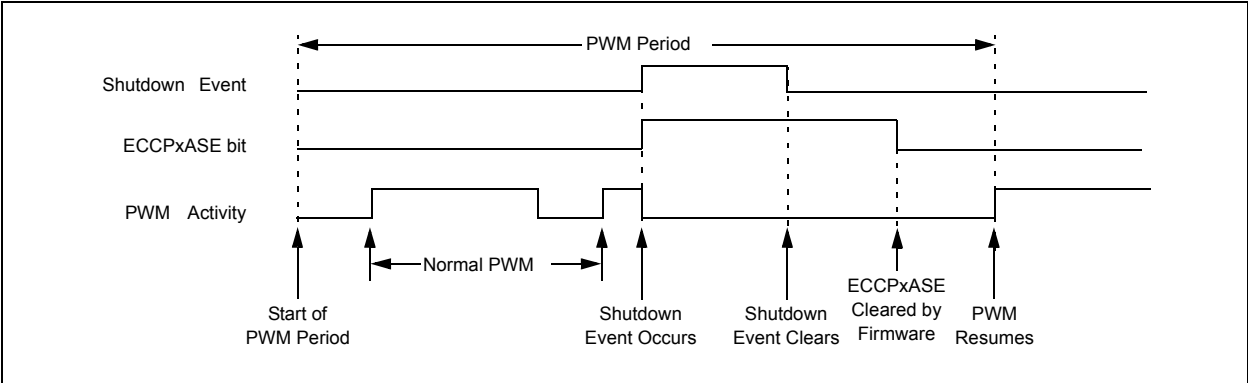
FIGURE 18-14: PWM AUTO-SHUTDOWN WITH FIRMWARE RESTART (PxRSEN = 0)
