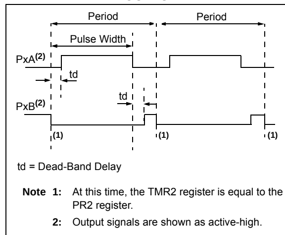
FIGURE 18-16: EXAMPLE OF HALF-BRIDGE PWM OUTPUT
