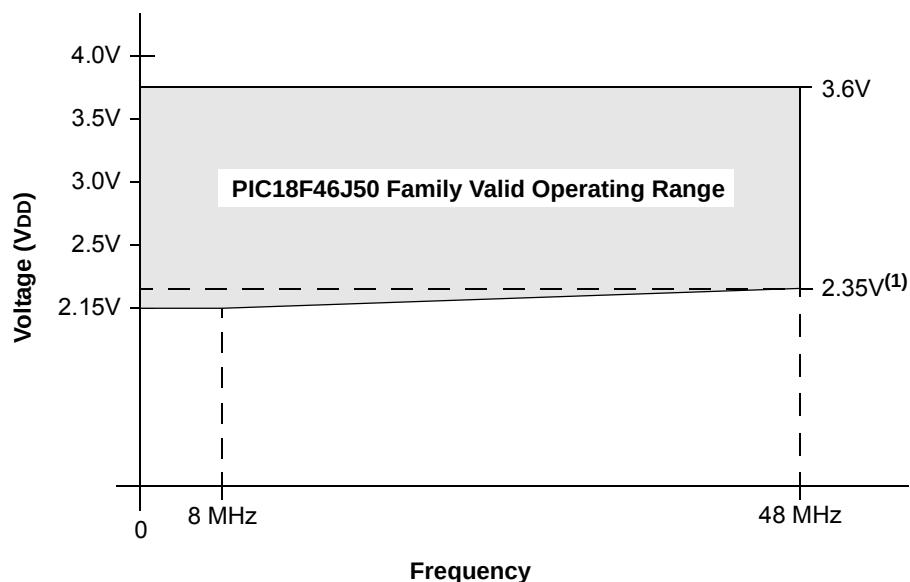
FIGURE 30-1: PIC18F46J50 FAMILY V_{DD} FREQUENCY GRAPH (INDUSTRIAL)
