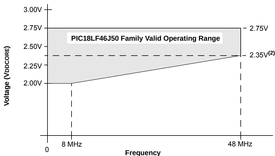
FIGURE 30-2: PIC18LF46J50 FAMILY V_{DDCORE} FREQUENCY GRAPH (INDUSTRIAL) (1)
