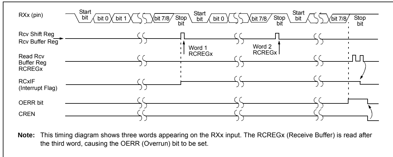
FIGURE 20-7: ASYNCHRONOUS RECEPTION
