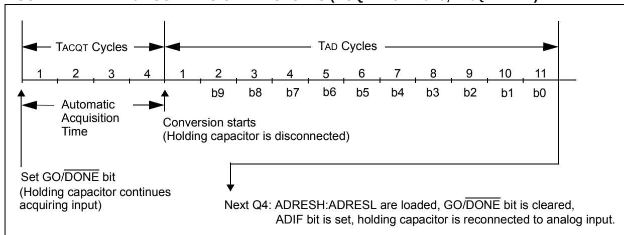
FIGURE 21-4: A/D CONVERSION TAD CYCLES ( \text{ACQT}<2:0> = 010 , \text{TACQ} = 4 \text{ TAD} )
