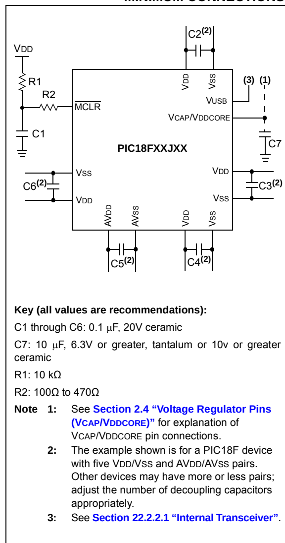
FIGURE 2-1: RECOMMENDED MINIMUM CONNECTIONS
