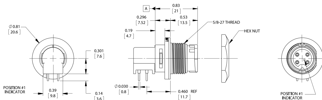
EN3® RIGHT ANGLE 2-8 POSITION MOLDED CONNECTORS
