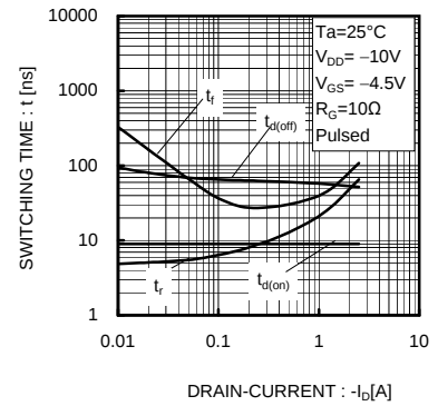
Fig.12 Switching Characteristics
