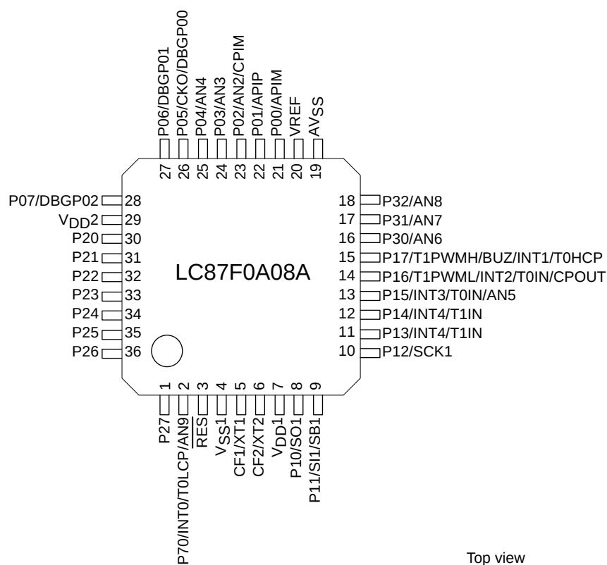
QFP36 (7×7) “Lead-free and halogen-free Type”
