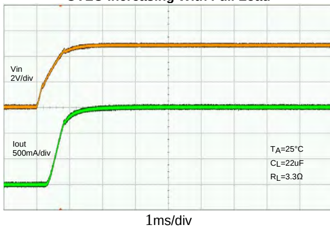
UVLO Increasing With Full Load
