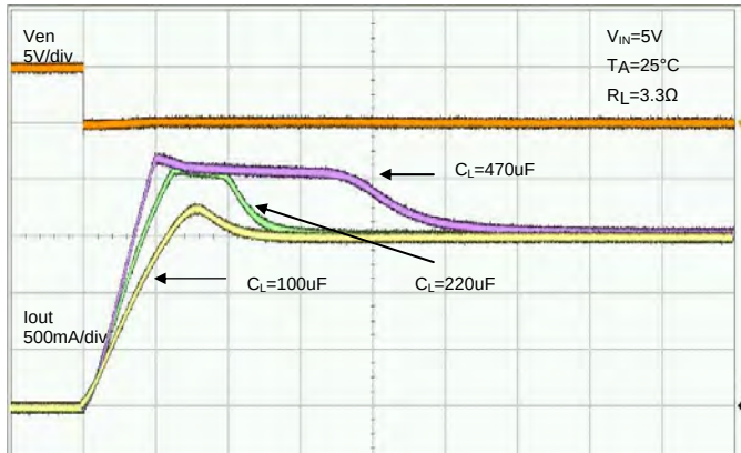
Inrush Current
