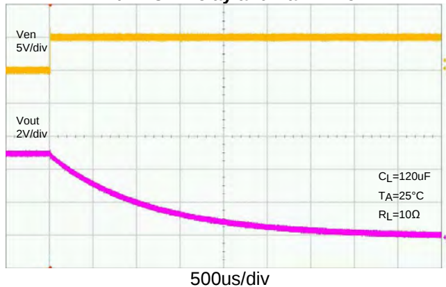
Turn-Off Delay and Fall Time
