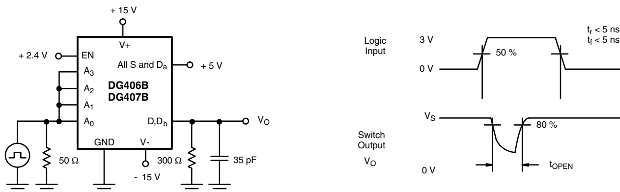
Fig. 4 - Break-Before-Make Interval
