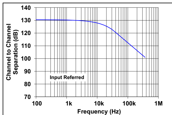
FIGURE 2-19: Channel-to-Channel Separation vs. Frequency (MCP6H82/4 only).
