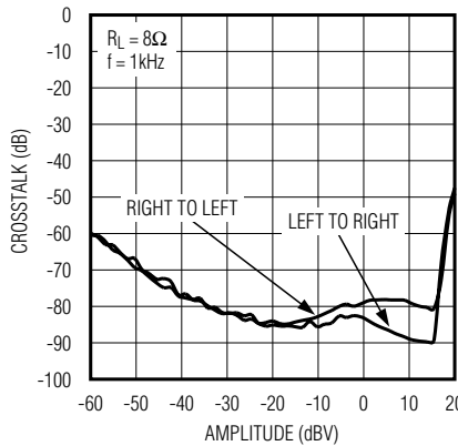
CROSSTALK vs. AMPLITUDE
