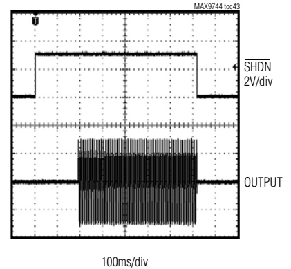
TURN-ON/OFF RESPONSE
