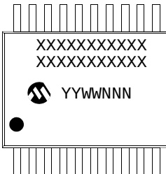
20-Lead SSOP (300 mil)
