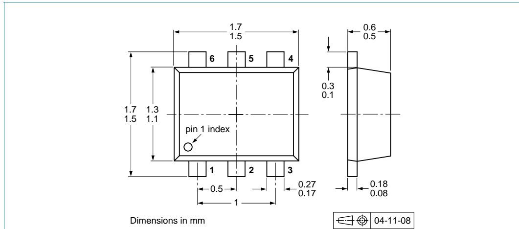
Fig 10. Package outline PEMH10 (SOT666)
