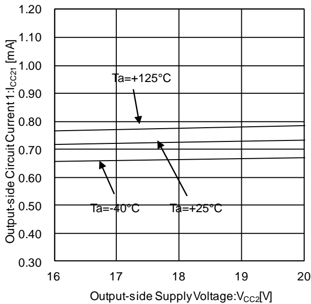
Figure 12. Output-side Circuit Current 2 vs Output-side Supply Voltage (At OUT=L)
