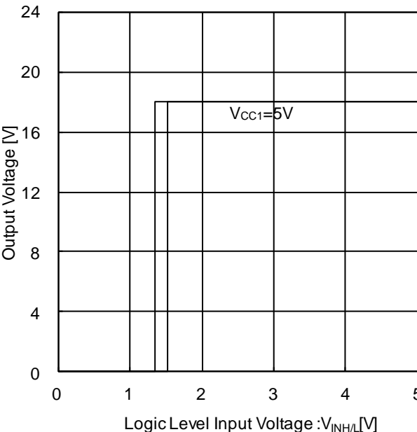
Figure 17. Output Voltage vs Logic Level Input Voltage (INA) (V<sub>CC1</sub>=5 V, V<sub>CC2</sub>=18 V, Ta=25 °C)
