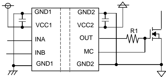
Figure 34. Driving SiC
