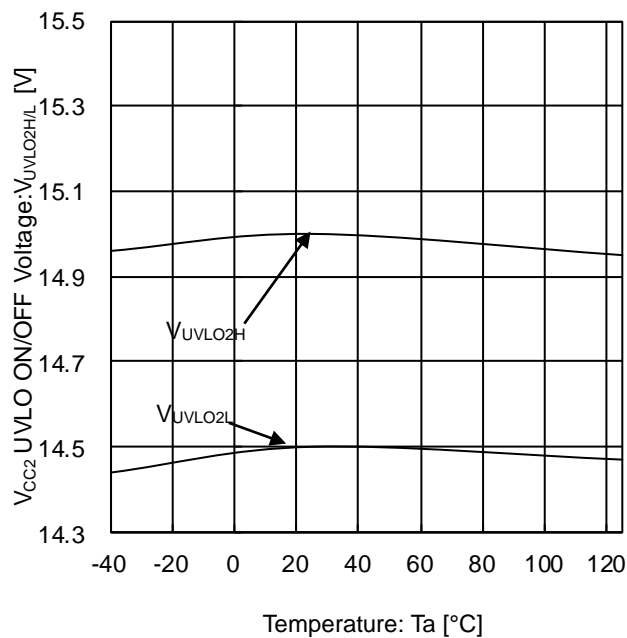
Figure 30 V CC2 UVLO ON/OFF Voltage vs Temperature
