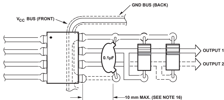
Figure 19. Recommended printed circuit board layout.
