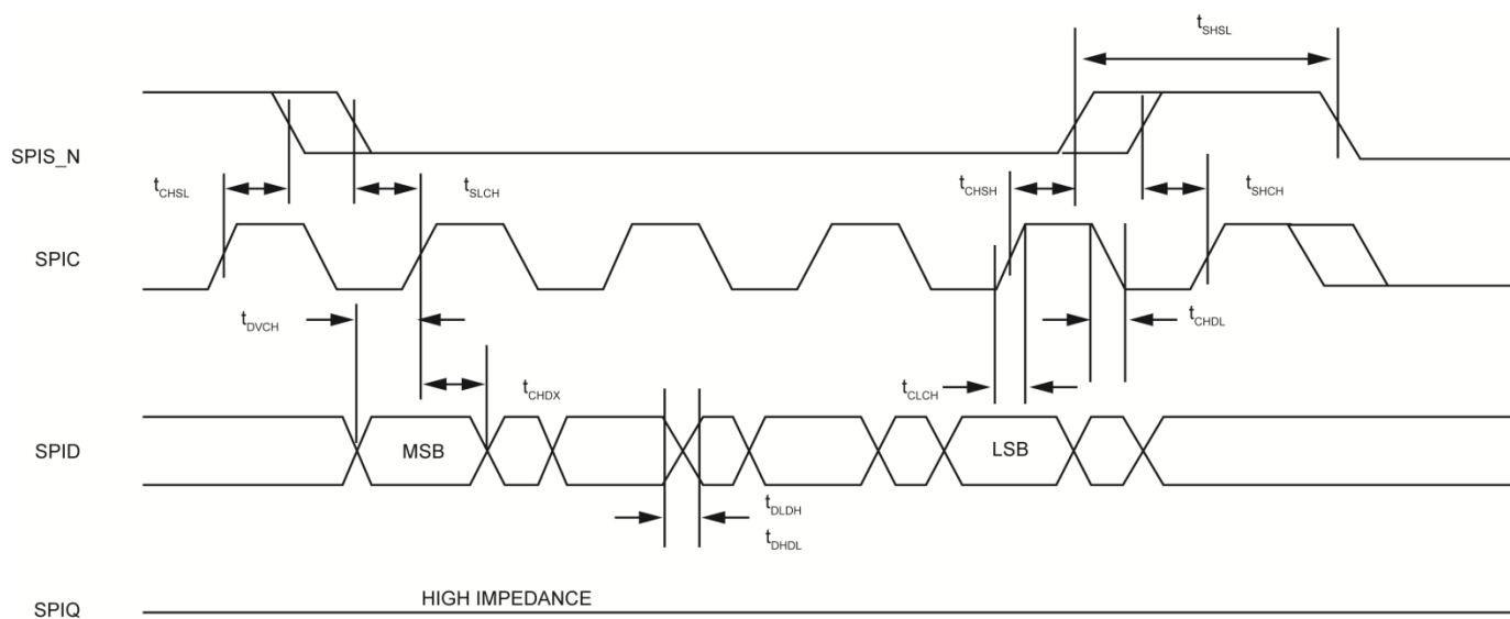
Figure 24. SPI Input Timing
