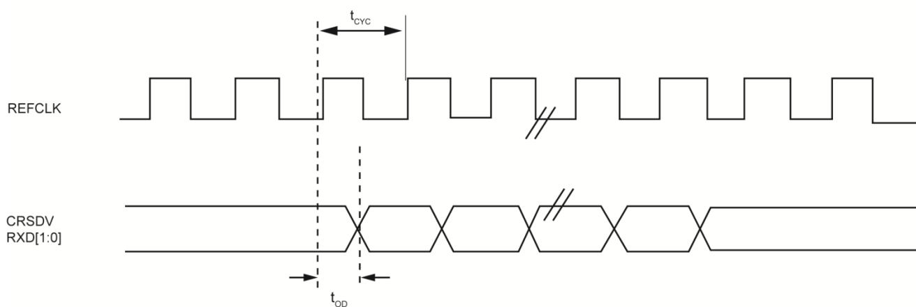
Figure 23. RMII Timing – Data Transmitted to RMII
