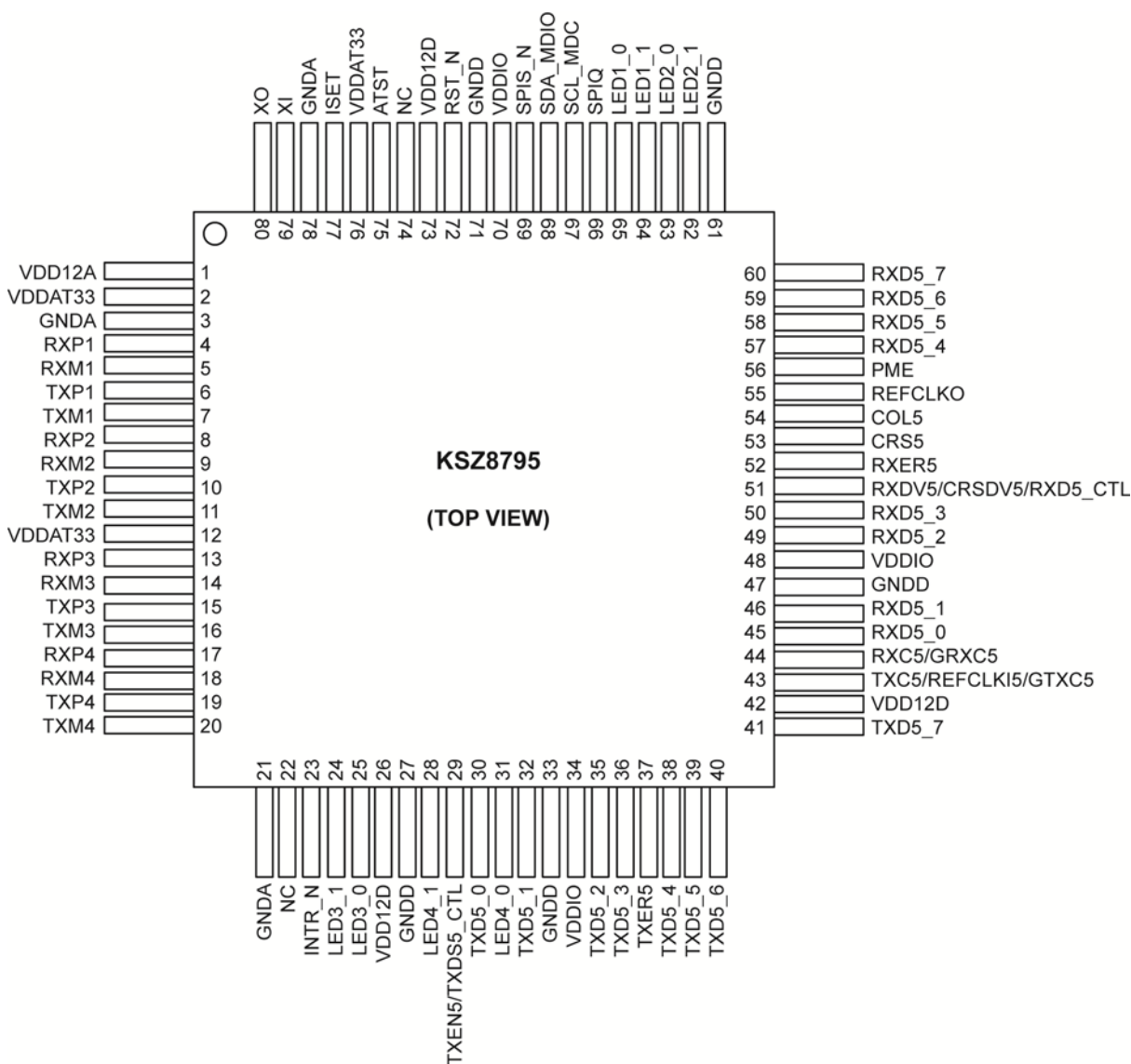
Figure 2. 80-Pin LQFP
