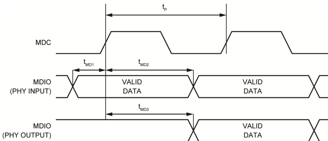
Figure 27. MDC/MDIO Timing
