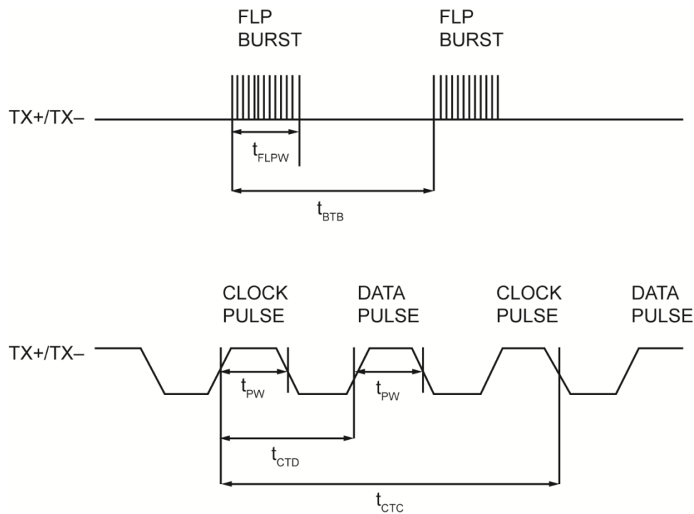
Figure 26. Auto-Negotiation Timing
