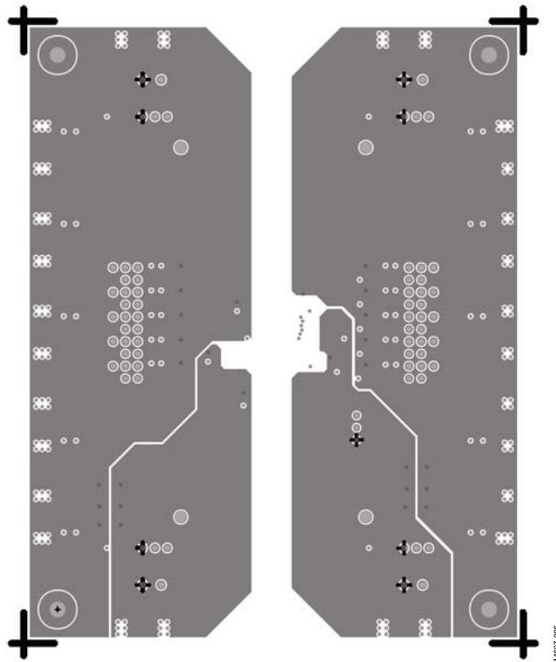
Figure 6. VDD1/VDDP/VDD2/ISO Power Planes (Layer 2)
