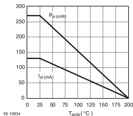
Figure 1. Derating diagram
