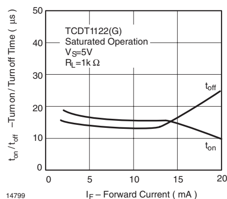
Figure 14. Turn on / off Time vs. Forward Current
