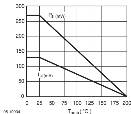
Figure 1. Derating diagram
