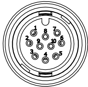
FACE VIEW
