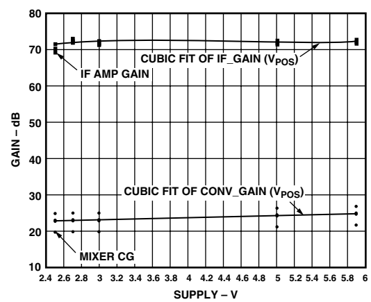
TPC 6. Mixer Conversion Gain and IF Amplifier Gain vs. Supply Voltage, T = 25^{\circ}\text{C} , V_{\text{GAIN}} = 0.3\text{ V} , V_{\text{REF}} = 1.5\text{ V} , I_{\text{F}} = 10.7\text{ MHz} , R_{\text{F}} = 250\text{ MHz}
