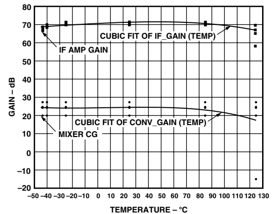
TPC 5. Mixer Conversion Gain and IF Amplifier Gain vs. Temperature, V_{\text{POS}} = 3\text{ V} , V_{\text{GAIN}} = 0.3\text{ V} , V_{\text{REF}} = 1.5\text{ V} , I_{\text{F}} = 10.7\text{ MHz} , R_{\text{F}} = 250\text{ MHz}
