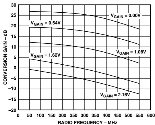
TPC 3. Mixer Conversion Gain vs. Frequency, T = 25^{\circ}\text{C} , V_{\text{POS}} = 2.92\text{ V} , V_{\text{REF}} = 1.35\text{ V} , I_{\text{F}} = 10.7\text{ MHz}
