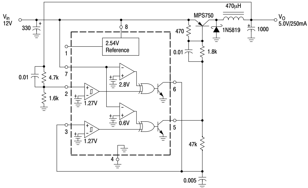
Figure 27. Step-Down Converter
