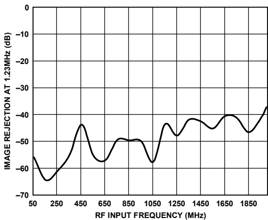
Figure 55. Image Rejection vs. RF Input Frequency for a CDMA2000 Signal, IF = 1.23 MHz
