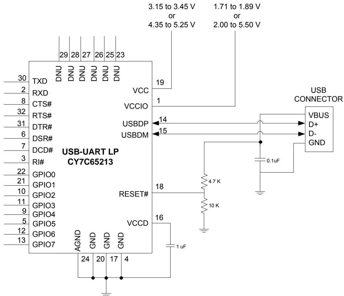
Figure 2. Self-Powered Configuration
