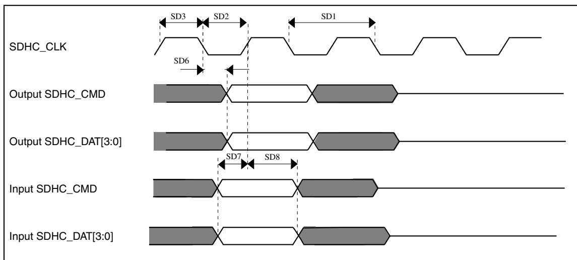
Figure 26. SDHC timing
