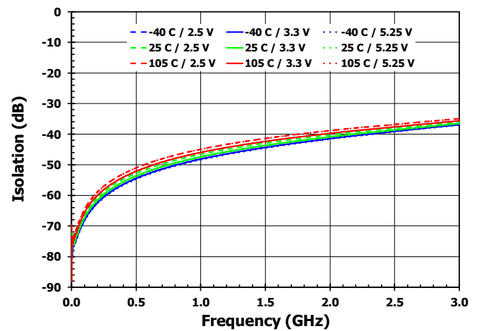
Figure 7. RF2 to RFC Isolation [RF1 On State]
