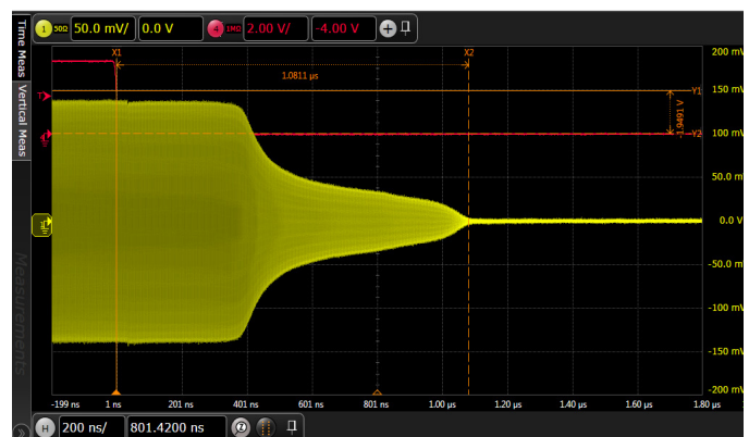
Figure 25. Switching Time [Insertion Loss to Isolation State]
