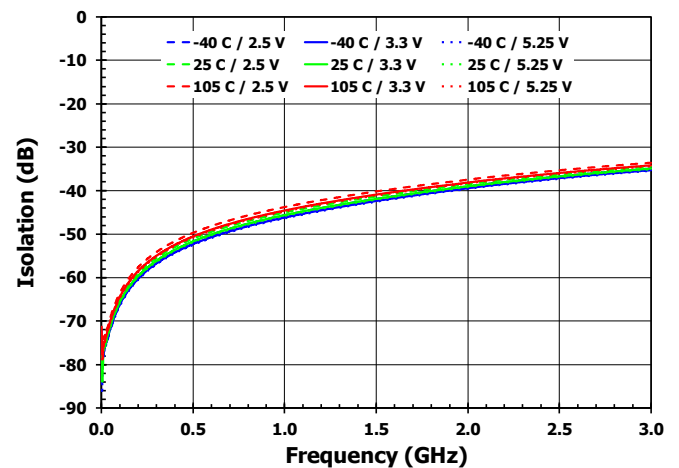
Figure 9. RF1 to RF2 Isolation [RF2 On State]
