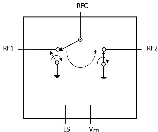
Figure 1. Block Diagram
