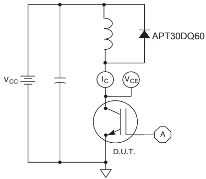
Figure 12, Inductive Switching Test Circuit
