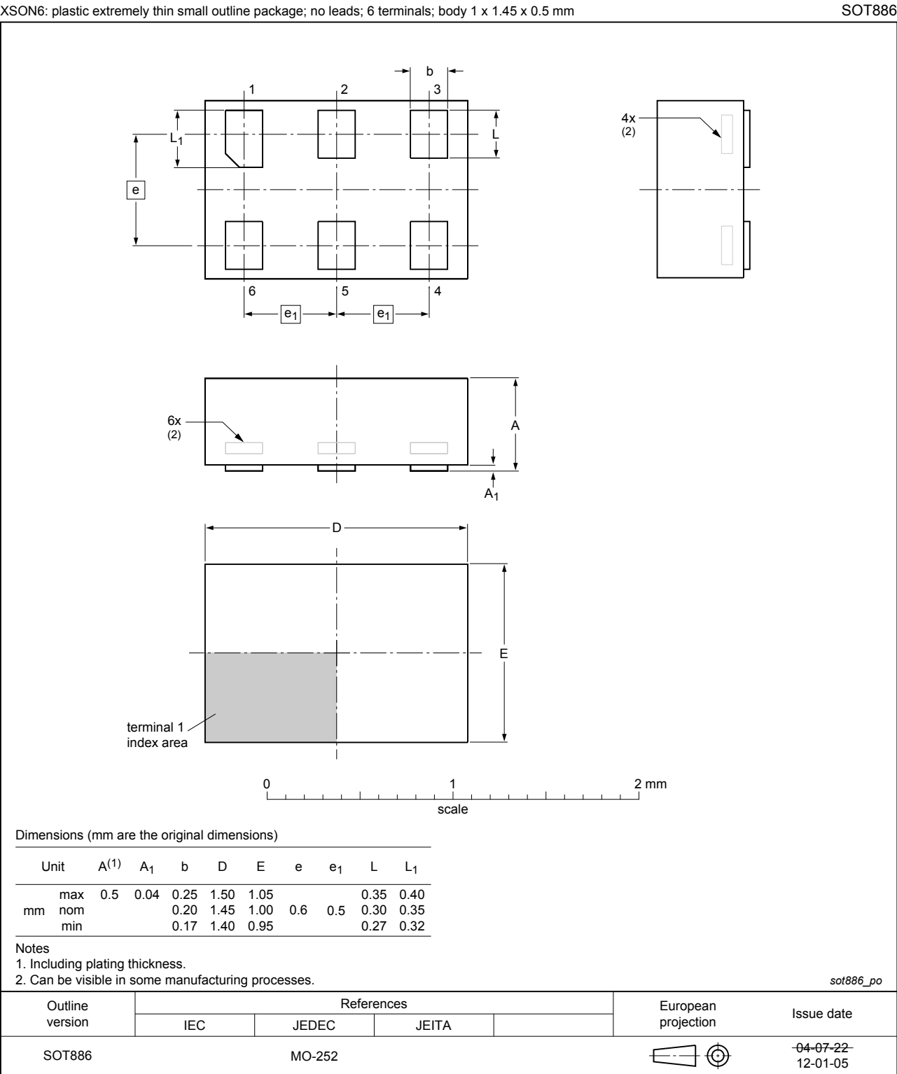
Figure 11. Package outline SOT886 (XSON6)
