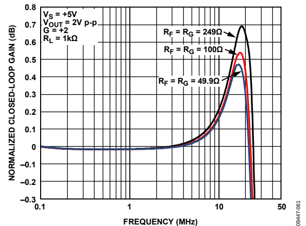
Figure 13. 0.1 dB Bandwidth at Selected R_F Values
