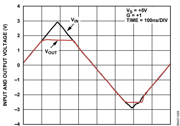
Figure 29. Input Overdrive Recovery Time
