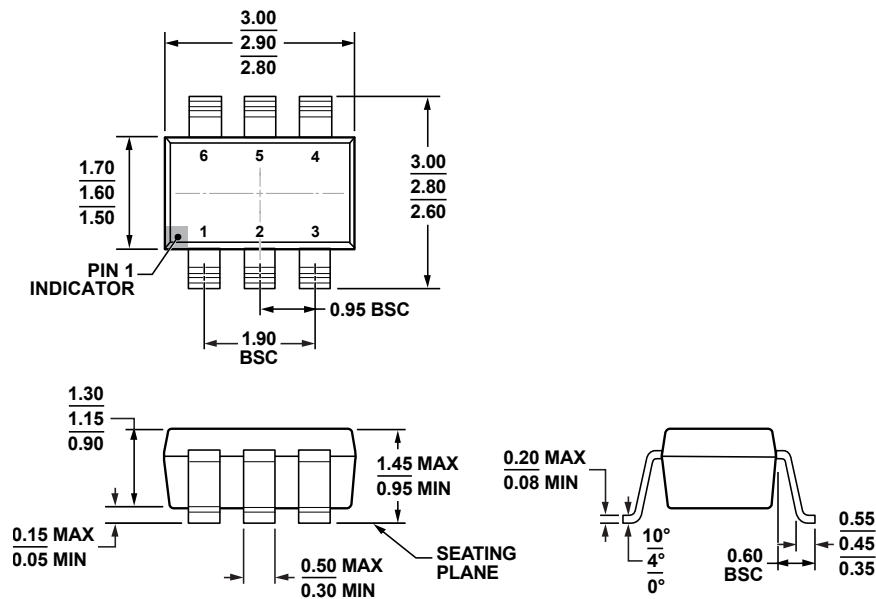
Figure 59. 6-Lead Small Outline Transistor Package [SOT-23] (RJ-6)
