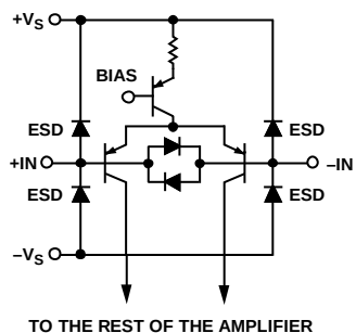
Figure 44. Input Stage and Protection Diodes
