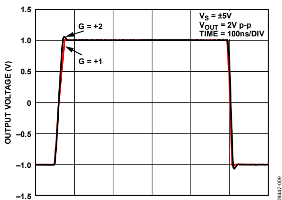
Figure 28. Large Signal Transient Response, G = +1 and G = +2
