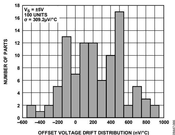
Figure 24. Input Offset Voltage Drift Distribution
