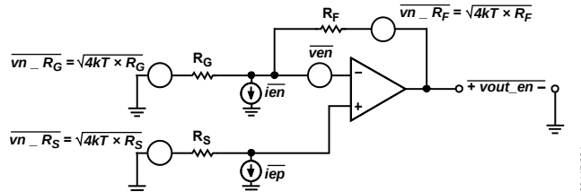
Figure 48. Noise Sources in Typical Connection
