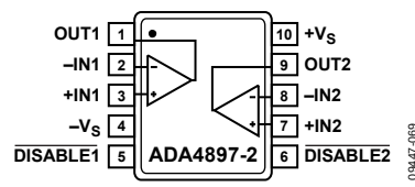
Figure 8. 10-Lead MSOP Pin Configuration
