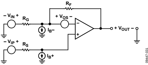
Figure 46. Typical Connection Diagram and DC Error Sources
