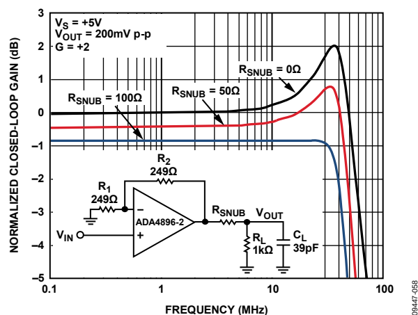
Figure 50. Using a Snub Resistor to Reduce Peaking Due to Output Capacitive Load
