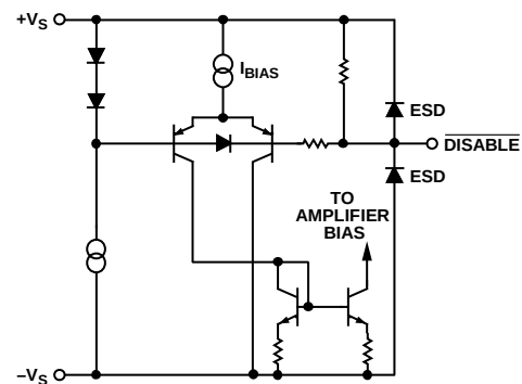
Figure 45. \overline{\text{DISABLE}} Circuit
