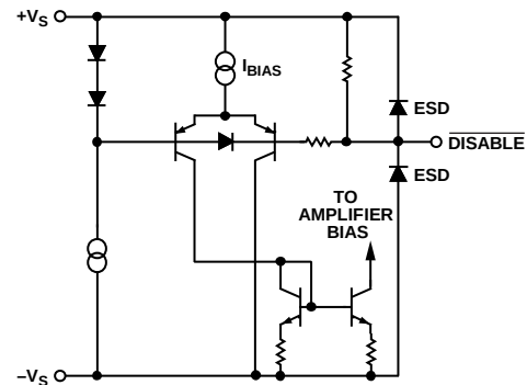
Figure 45. \overline{\text{DISABLE}} Circuit
