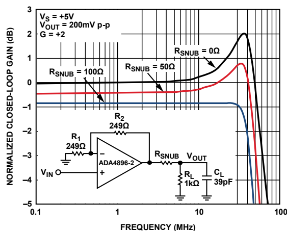
Figure 50. Using a Snub Resistor to Reduce Peaking Due to Output Capacitive Load
