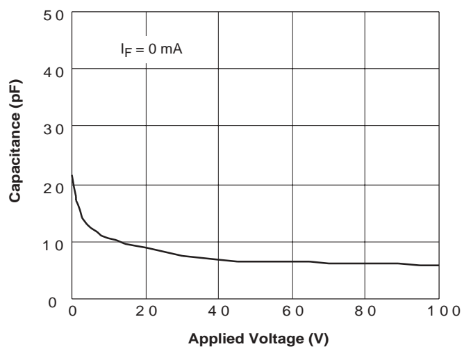
Figure 12. Switch Capacitance vs. Applied Voltage
