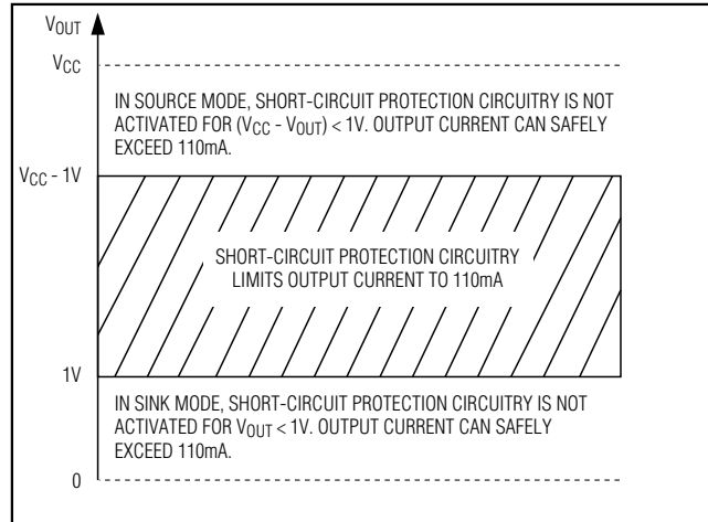
Figure 7. Short-Circuit Protection
