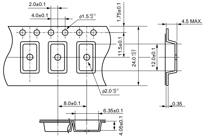
Outline and Dimensions (Tape)
