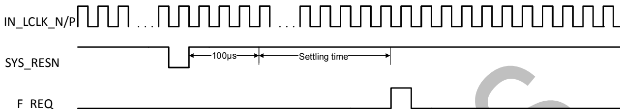
Figure 9: Reset sequence
