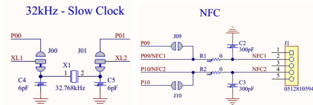
Figure 15 – GPIOs disconnected from I/O headers
