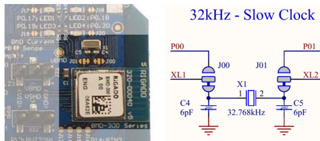
Figure 12 – Schematic - 32KHz Crystal
