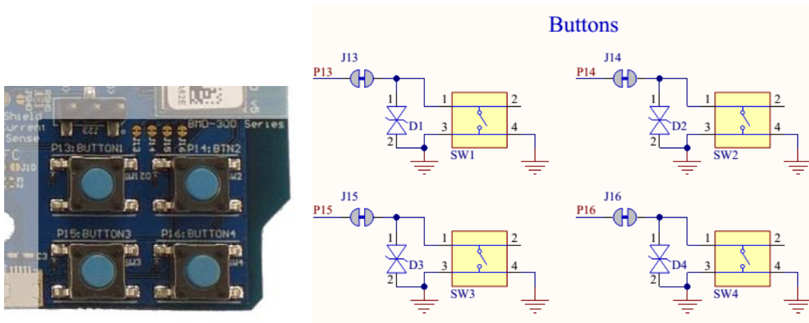
Figure 10 – Schematic – User Buttons
