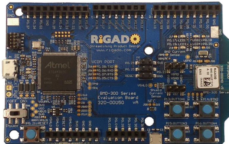
Figure 1 – BMD-300 Evaluation Board (Top View)
