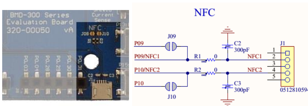
Figure 13 – NFC Connector
