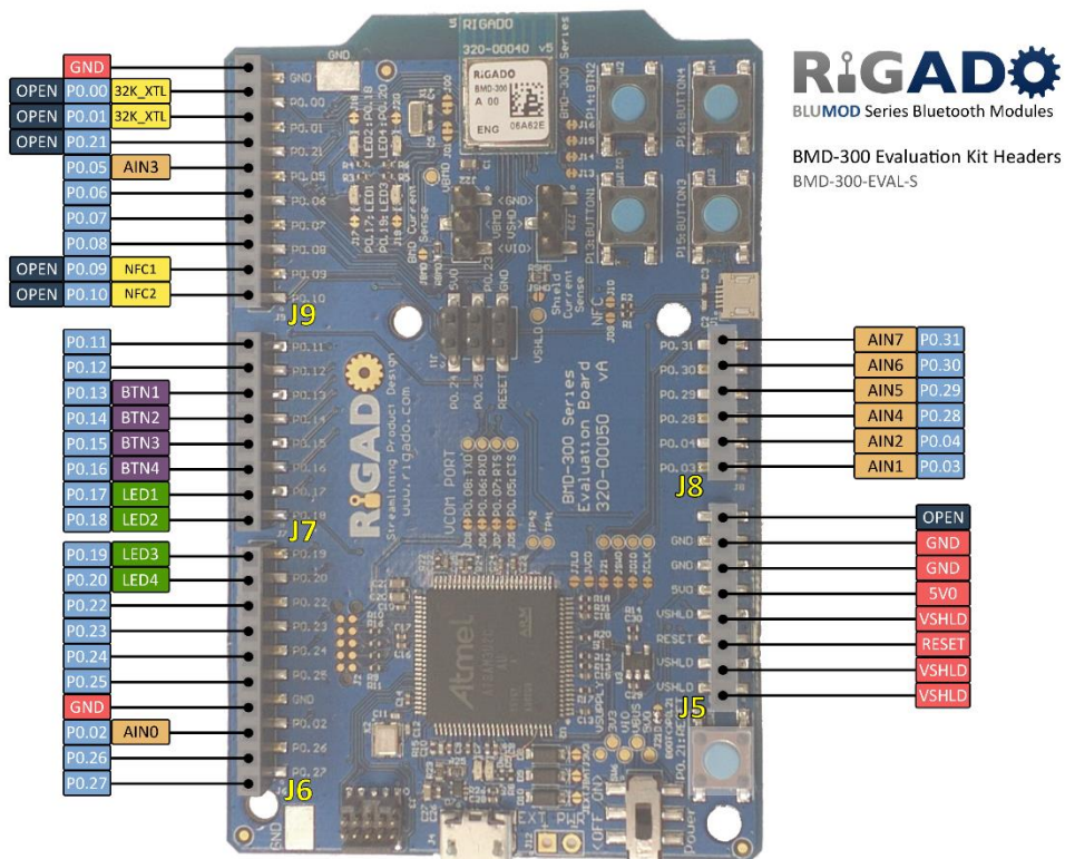
Figure 17 – BMD-300 Series Evaluation Board Pin-out
