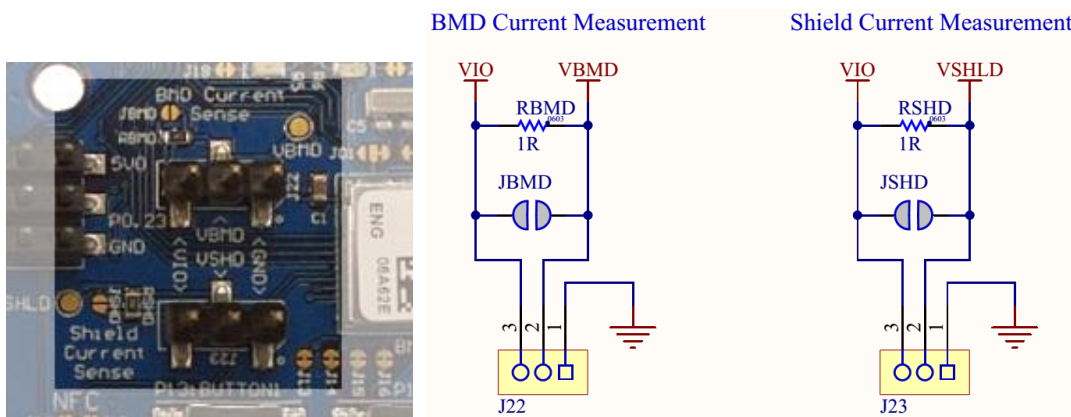
Figure 14 – Current Sensing Header Layout
