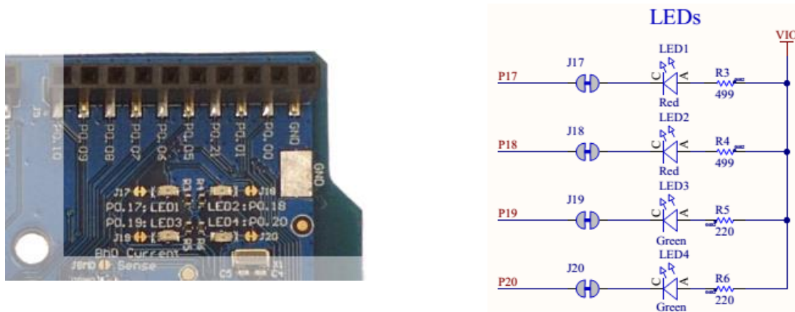
Figure 11 – Schematic – User LEDs
