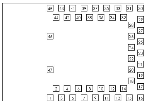
Figure 18 – BMD-300 Series Module Pin-out
