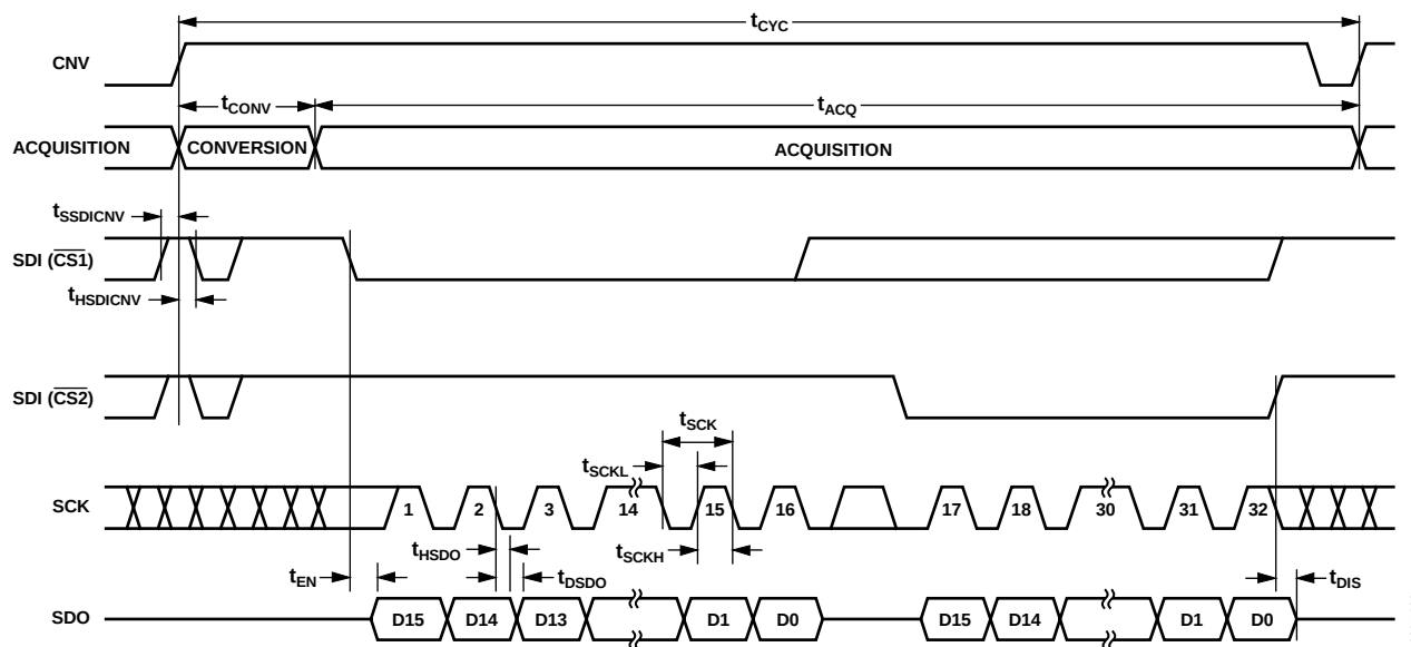
Figure 37. 4-Wire CS Mode Serial Interface Timing
