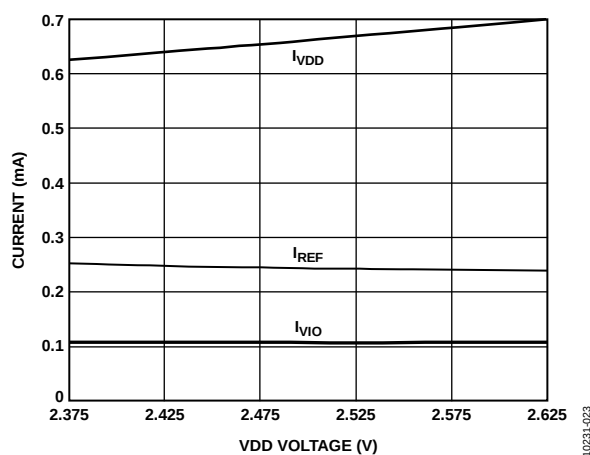
Figure 22. Operating Currents vs. Supply (AD7988-5)
