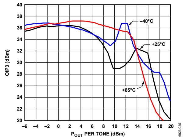
Figure 20. OIP3 vs. Output Power ( P_{OUT} ) and Temperature
