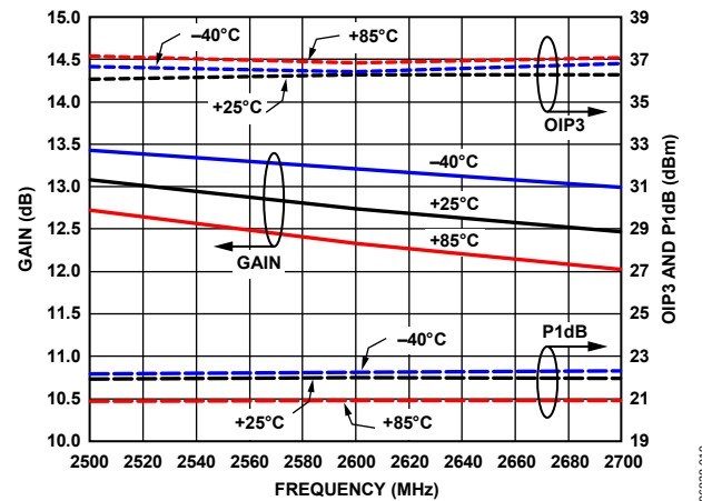
Figure 19. Gain, OIP3, and P1dB vs. Temperature
