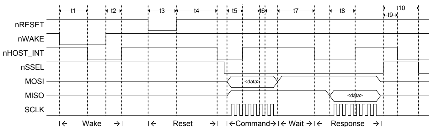
Figure 7. SPI Protocol Timing Waveform
