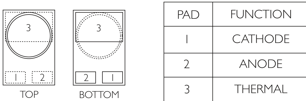
Figure 2. Pad configuration.
