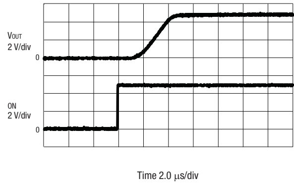
Figure 10. AAT4616IPS-1 and AAT4616IGV-1 Turn-On ( R_L = 10\ \Omega , C_L = 0.47\ \mu F )
