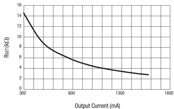
Figure 8. R_{SET} vs I_{LM} ( T_A = 25\text{ }^{\circ}\text{C} )
