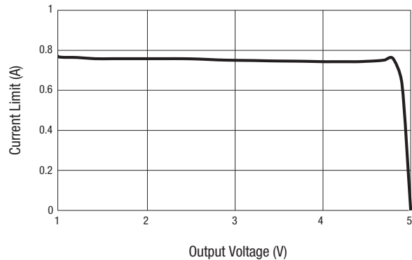
Figure 4. Current Limit vs Output Voltage ( V_{IN} = 5.0\text{ V} , T_A = 25\text{ }^{\circ}\text{C} , R_{SET} = 6.04\text{ k}\Omega )
