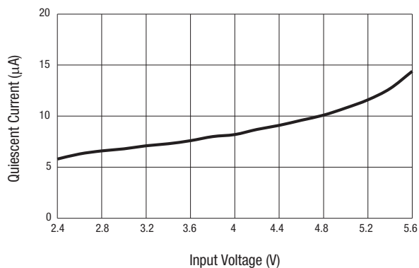
Figure 5. Quiescent Current vs Input Voltage ( T_A = 25\text{ }^{\circ}\text{C} )
